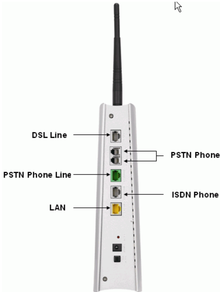
Figure 2 Splitterless type
