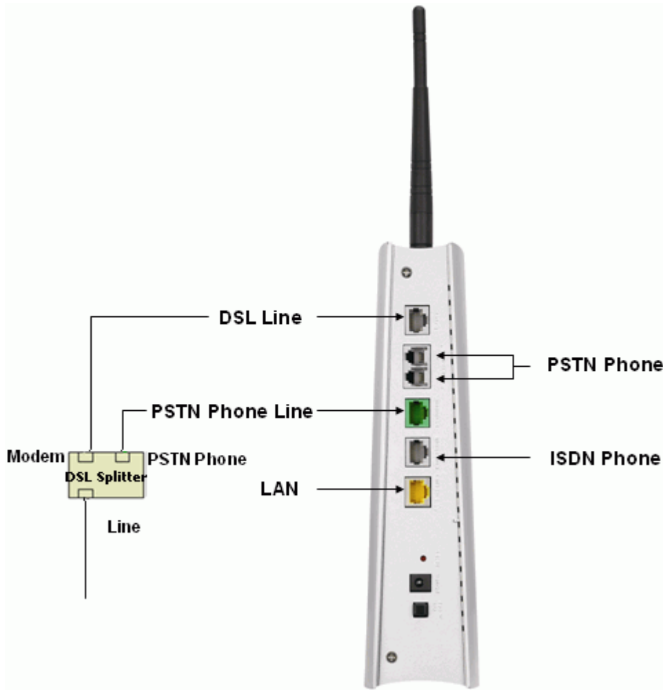
Figure 1 Splitter type
