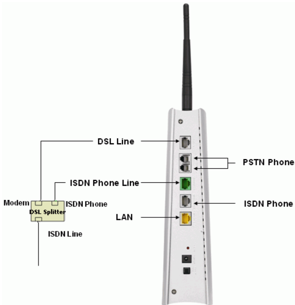
Figure 1 Splitter type
