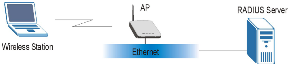
Figure 6-8 EAP Authentication
