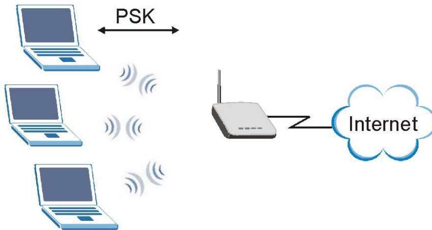
Figure 6-9 WPA-PSK Authentication
