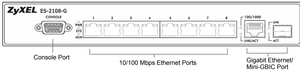
Figure 10 Front Panel: ES-2108-G/ES-2108PWR
