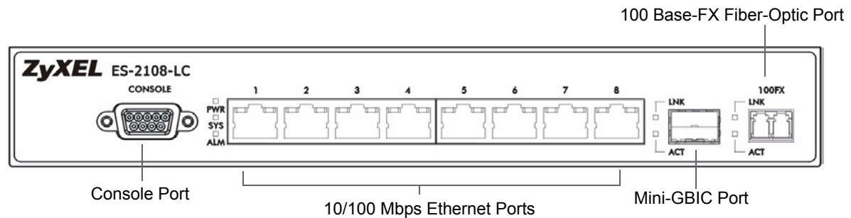
Figure 11 Front Panel: ES-2108-LC
