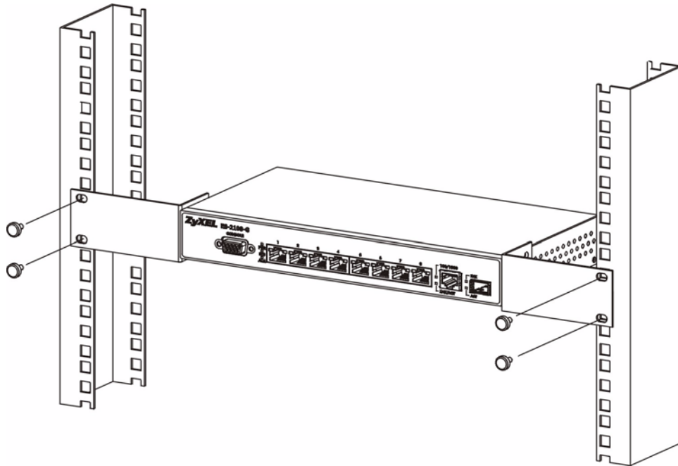
Figure 8 Mounting the Switch on a Rack
