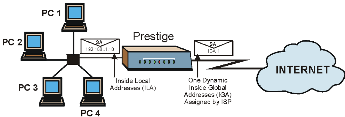
Figure 19-11 NAT Example 1
