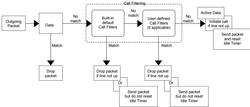
Figure 20-1 Outgoing Packet Filtering Process
