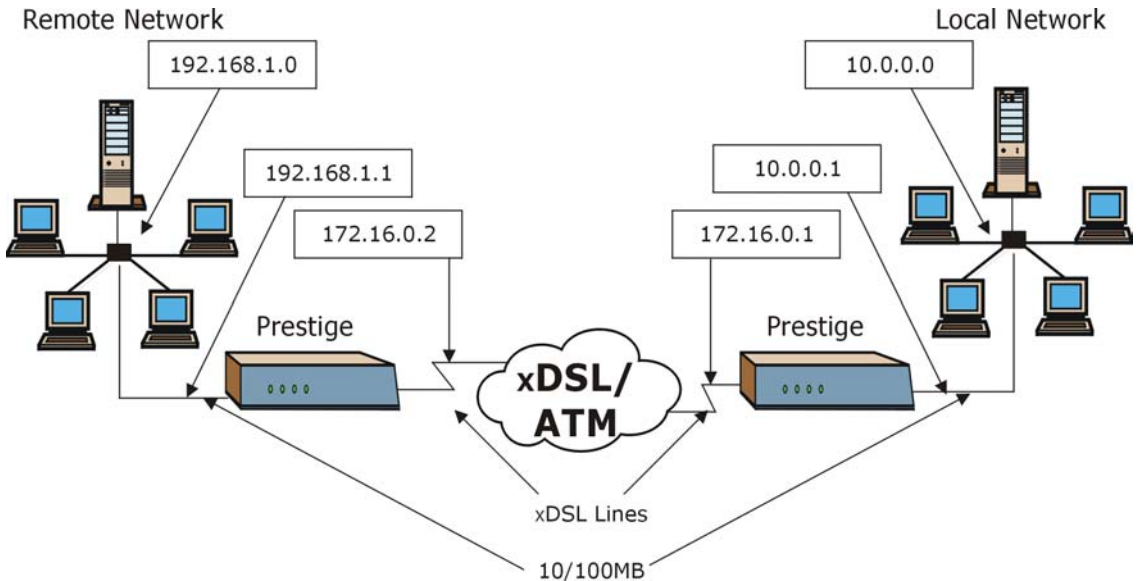
Figure 16-4 Sample IP Addresses for a TCP/IP LAN-to-LAN Connection
