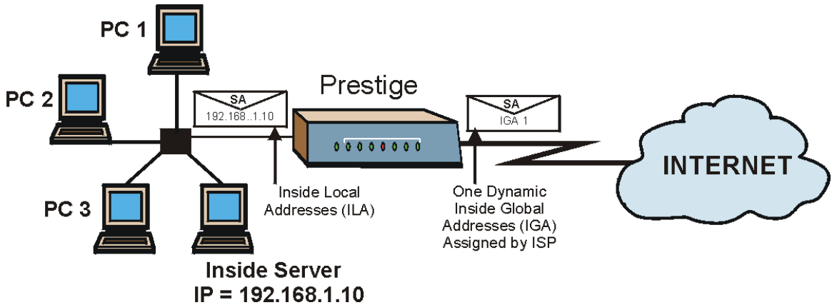
Figure 19-13 NAT Example 2
