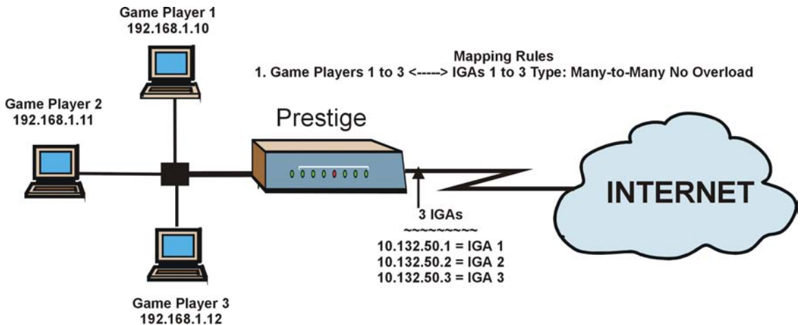
Figure 19-19 NAT Example 4
