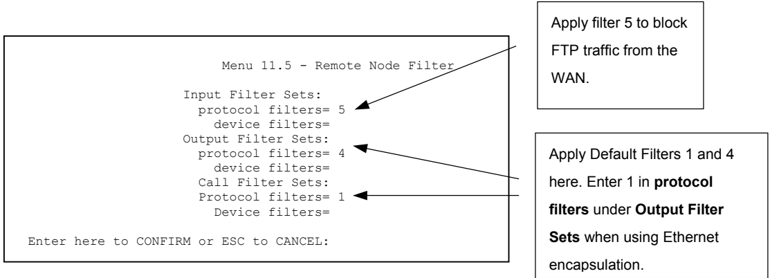
Figure 20-17 Filtering Remote Node Traffic
