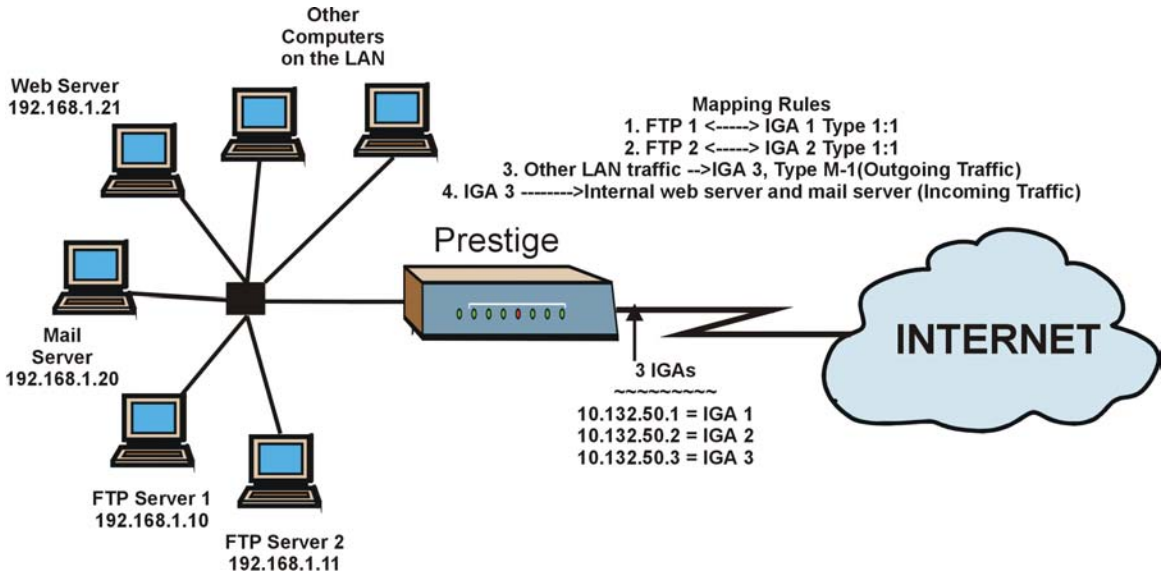
Figure 19-15 NAT Example 3
