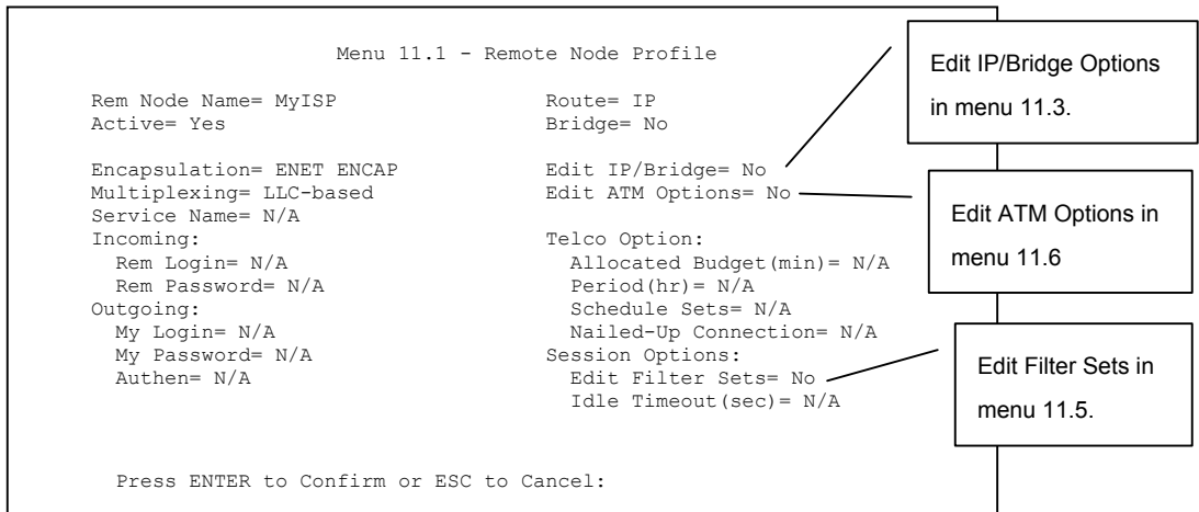
Figure 16-2 Menu 11.1 Remote Node Profile
