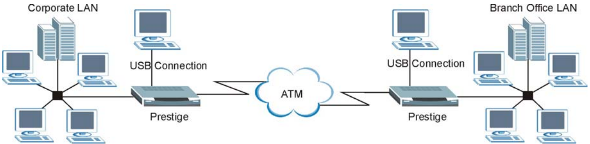
Figure 1-2 LAN-to-LAN Application
