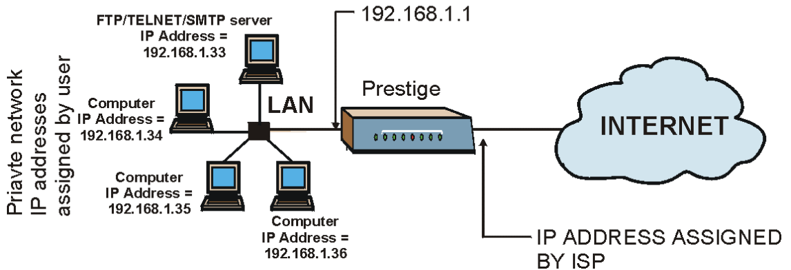
Figure 19-10 Multiple Servers Behind NAT Example
