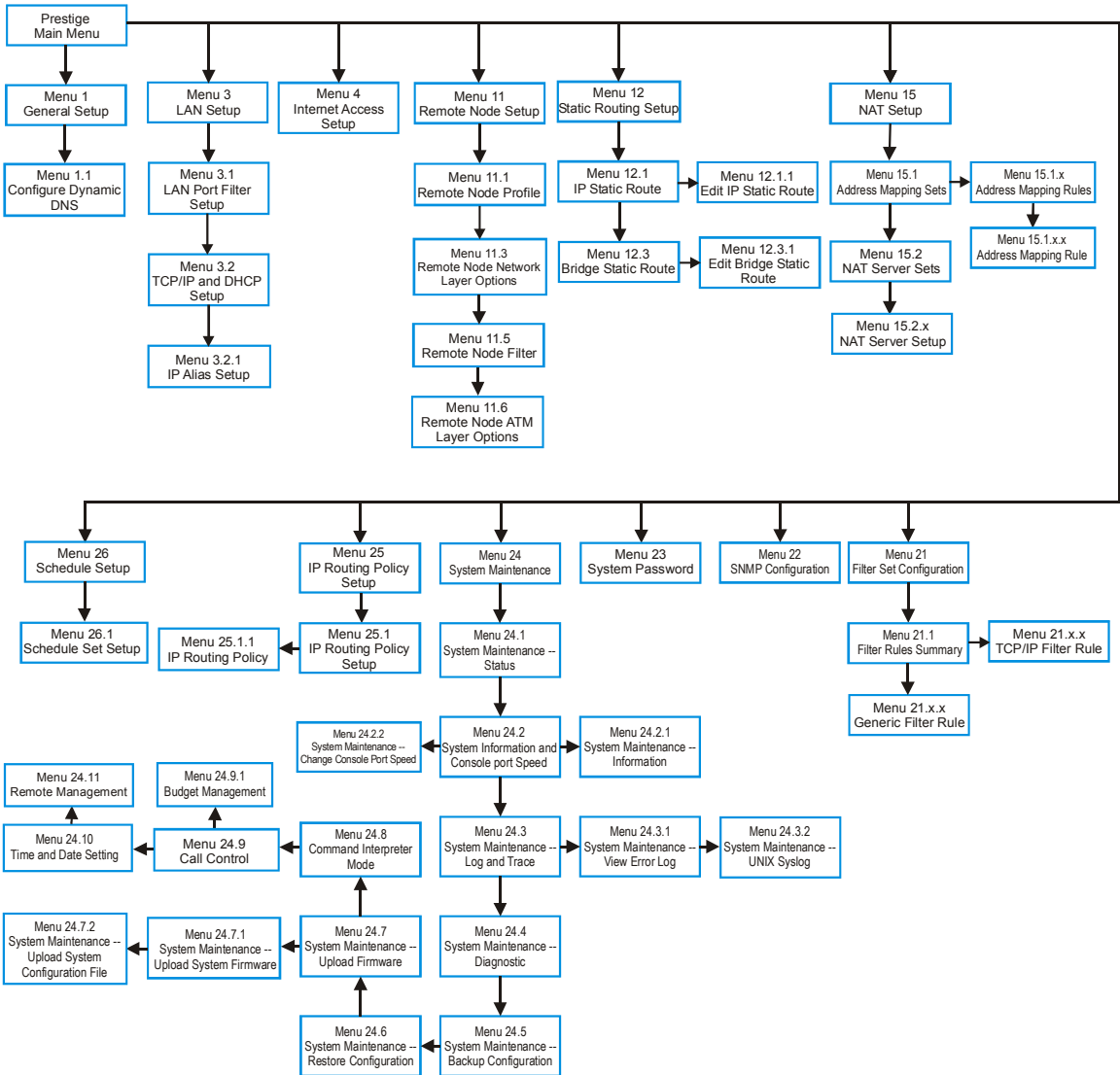
Figure 12-2 Prestige 623R-T SMT Menu Overview
