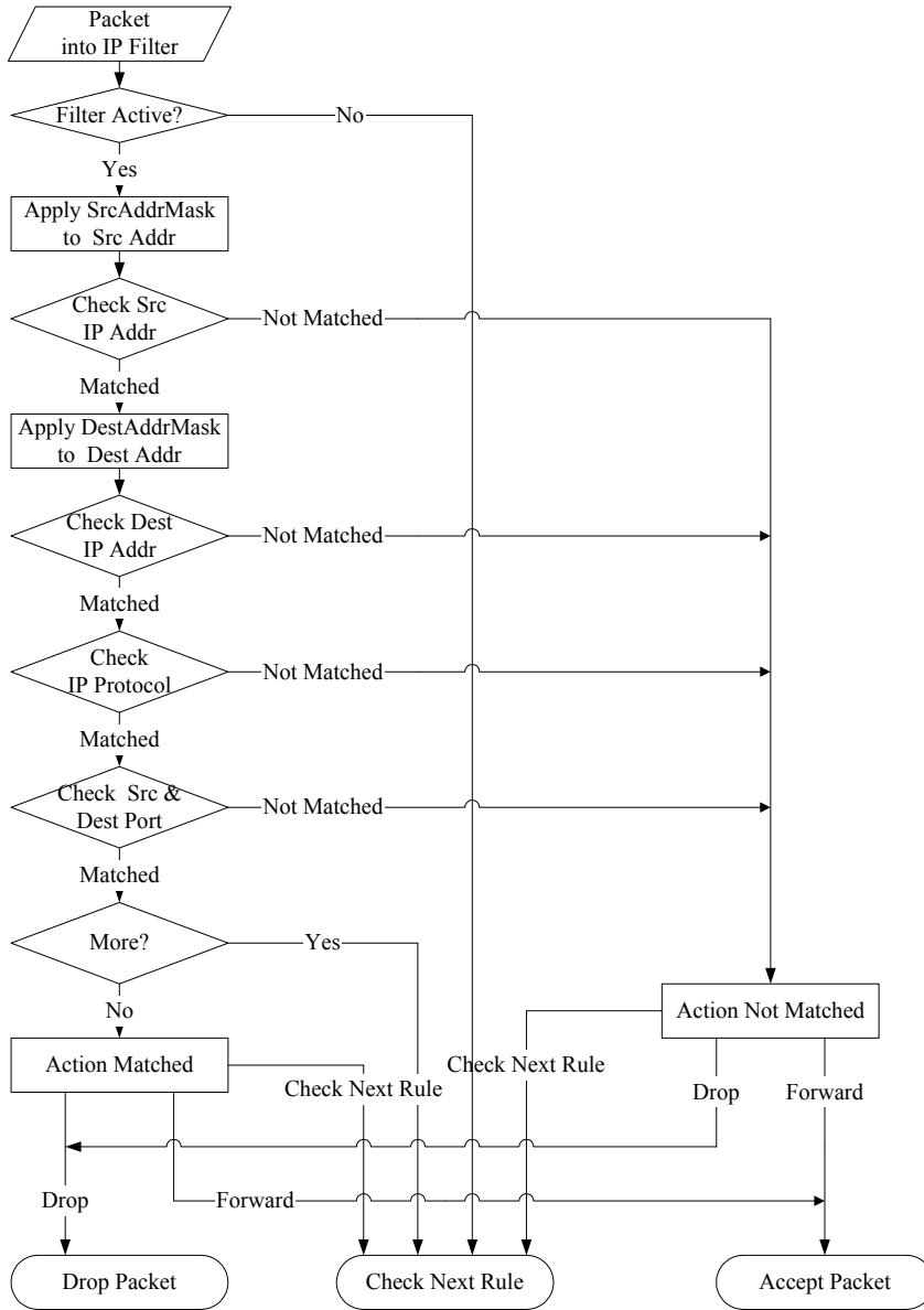
Figure 20-10 Executing an IP Filter
