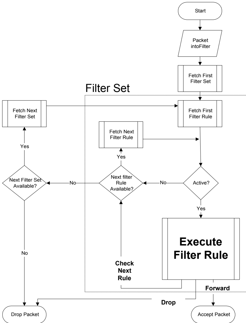
Figure 20-2 Filter Rule Process
