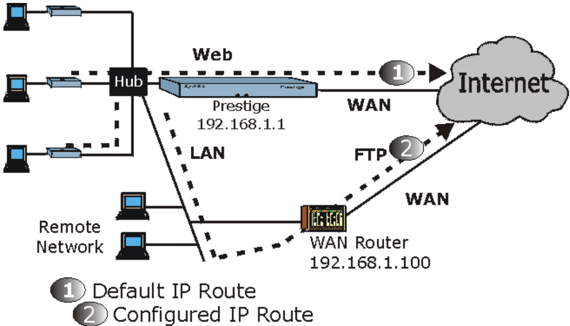
Figure 26-6 Example of IP Policy Routing
