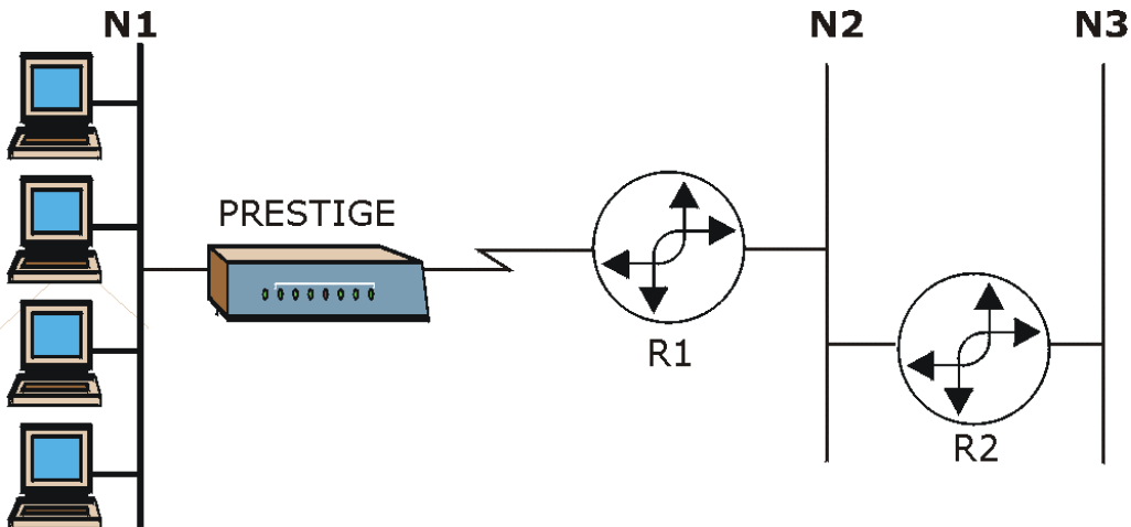
Figure 17-1 Sample Static Routing Topology
