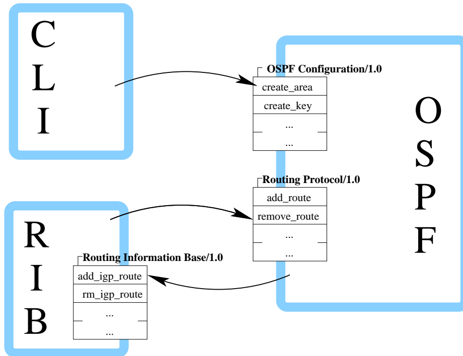
Figure 1: Example XRL Targets and clients: OSPF, RIB, and CLI. OSPF and RIB processes are XRL targets. OSPF supports XRL interfaces “OSPF Configuration/1.0” and “Routing Protocol/1.0”: the CLI is a client of the “OSPF Configuration/1.0” interface and the RIB a client of the “Routing Protocol/1.0” interface. RIB supports XRL interface “Routing Information Base/1.0”: the OSPF is a client of that interface.
